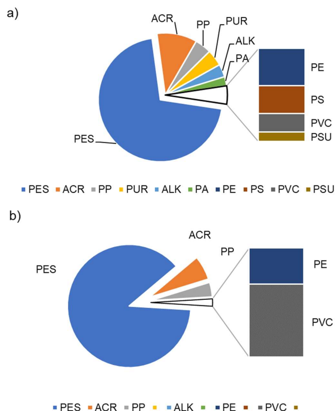
Figure 3. Chemical composition (percentages) of atmospheric MP deposition identified in this work. All types (a) and only fibres (b): Polyester (PES), acrylic polymers (ACR), polypropylene (PP), polyurethane (PUR), alkyd resins (ALK), polyamide (PA), polyethylene (PE), polystyrene (PS), polyvinyl chloride (PVC) and polysulfone (PSU).
